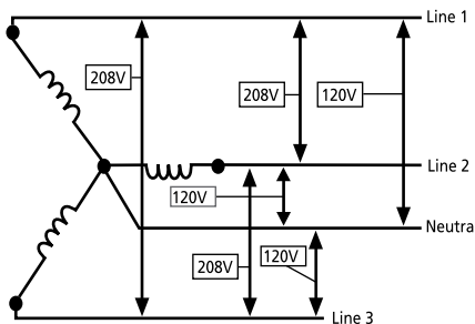
Figure 3: Three-Phase Wiring Diagram
